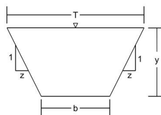
Figure 5.6-3. Trapezoid Dimensions
