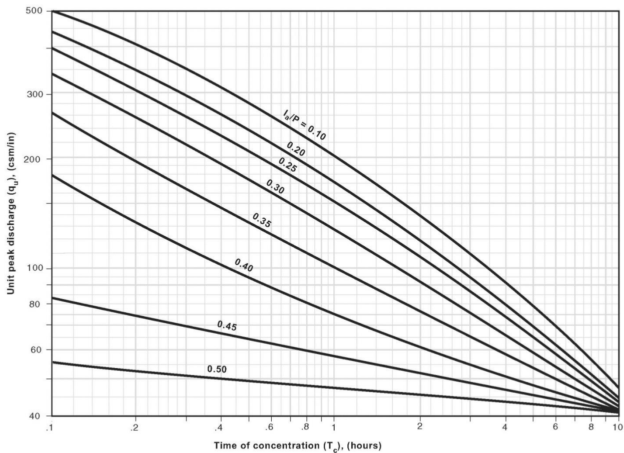
Figure B-1: Unit Peak Discharge ( q_u ) for NRCS (SCS) Type I Distribution
