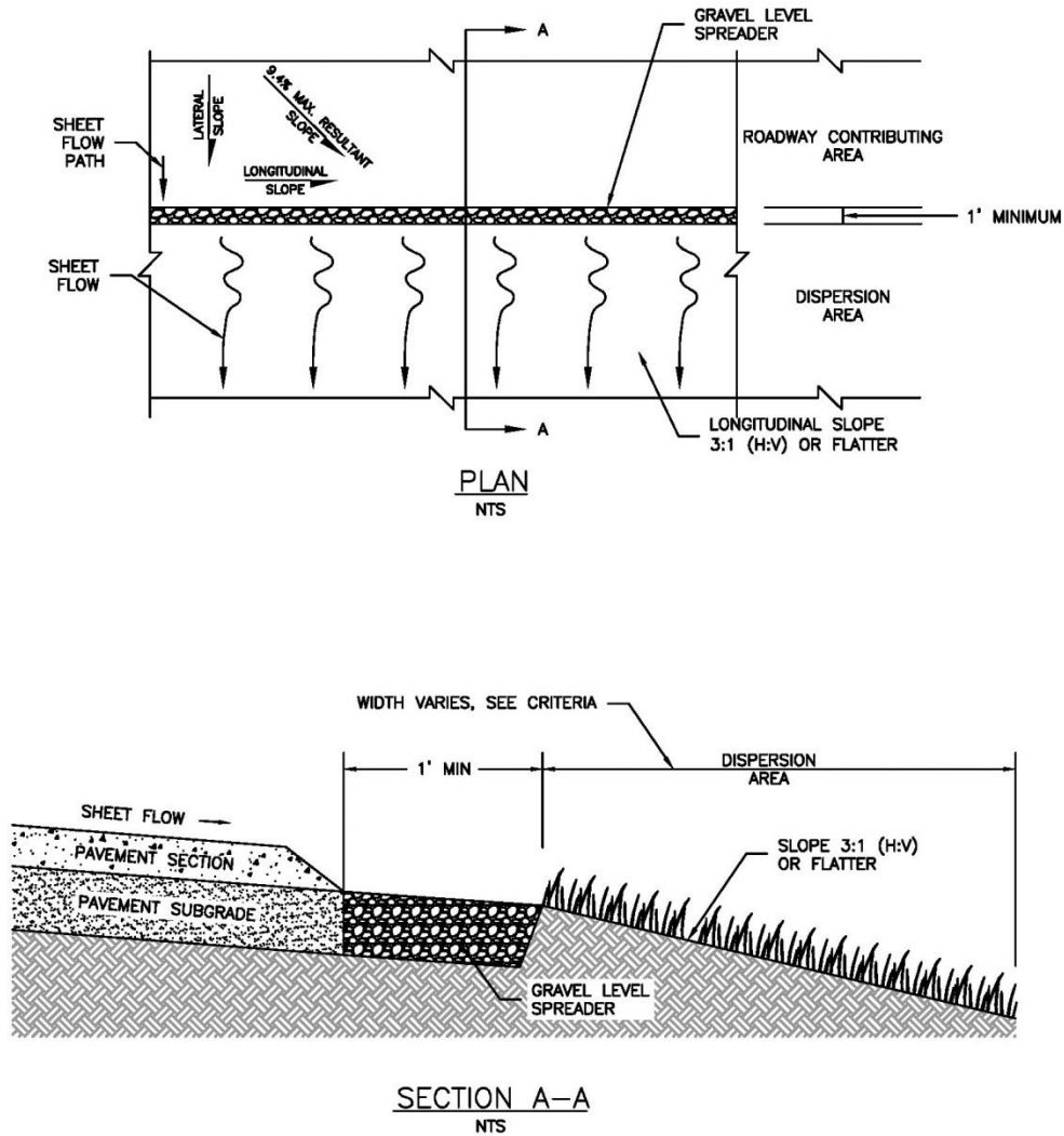
Figure 5.5-3. Dispersion Plan View and Typical Section
