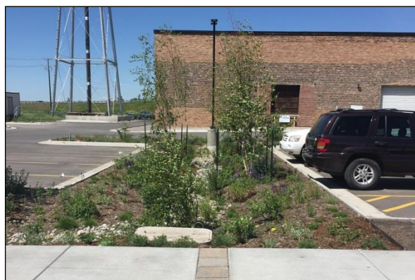
Figure 5.3-1. Bioretention Area
