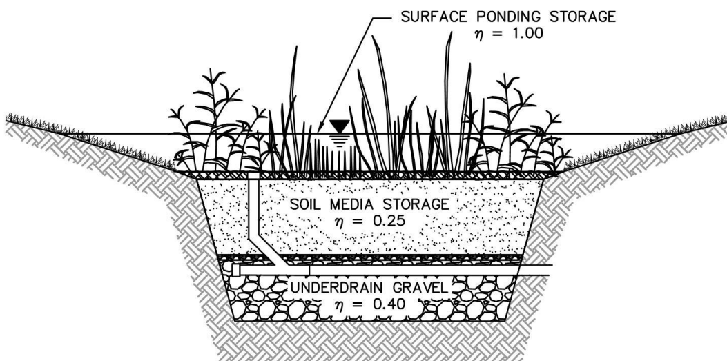
Figure 5.3-4. Bioretention Section with Typical Porosity Values
