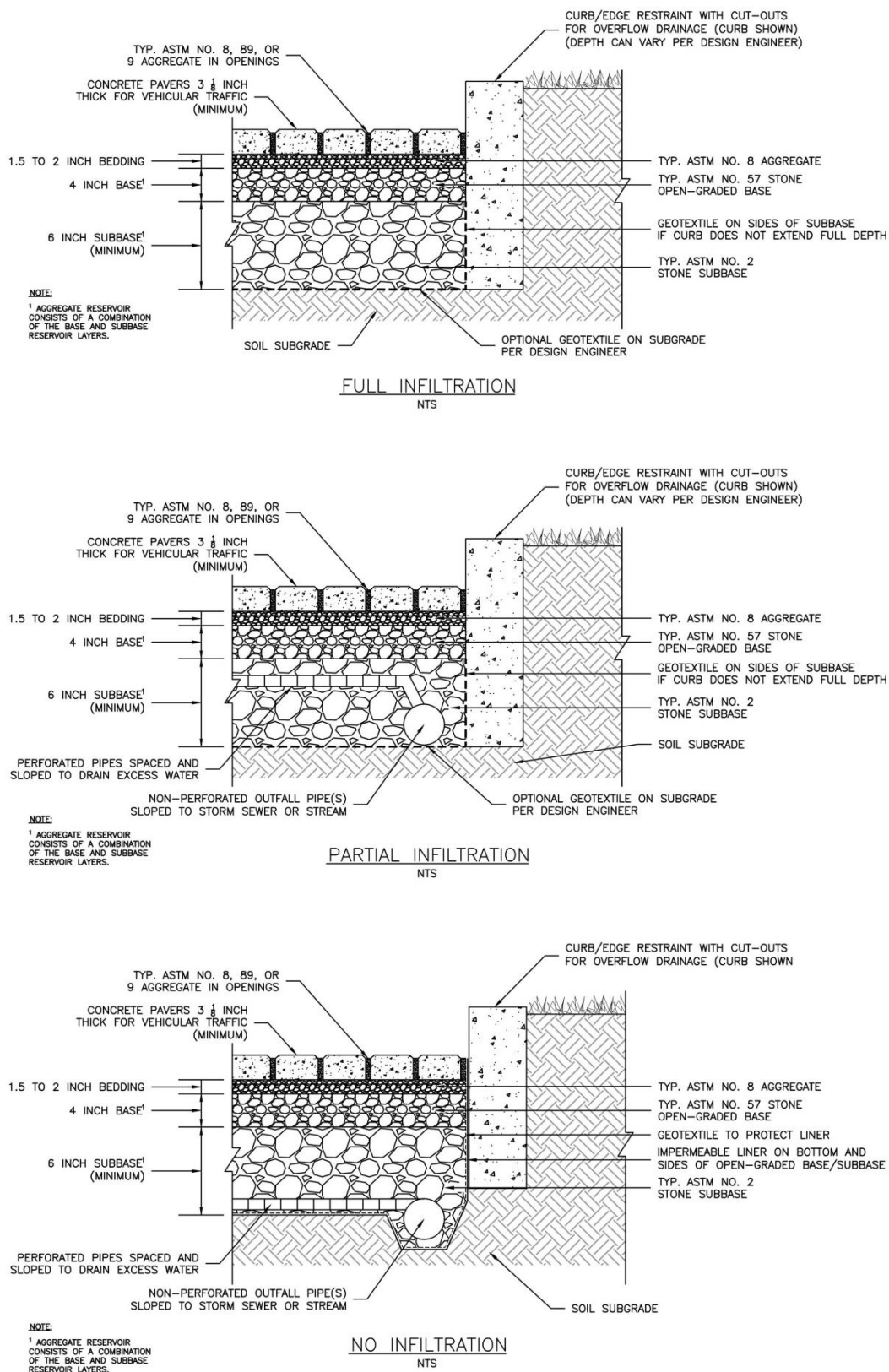
Figure 5.4-9. Full, Partial, and No Infiltration Sections
